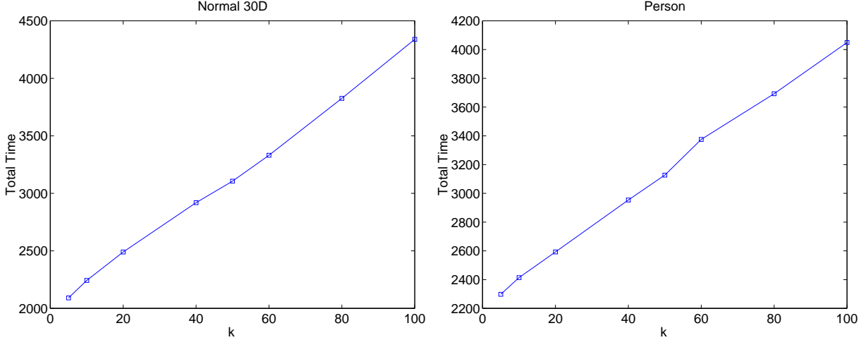
Figure 2: Total time (CPU and I/O) taken to mine outliers as k increases for the data sets Normal 30D and Person (with N = 1,000,000 ).
